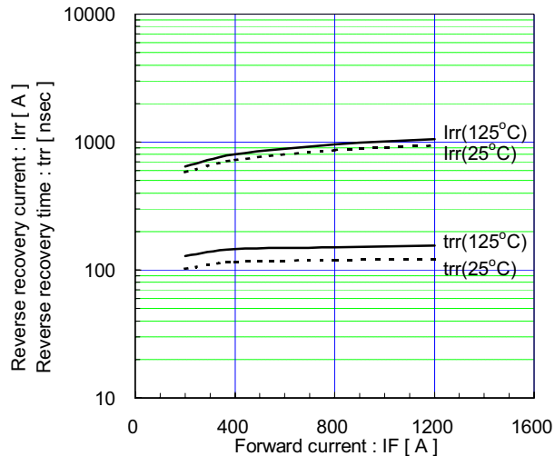
Reverse recovery characteristics (typ.) Vcc=600V, VGE=±15V, RG=0.68Ω
