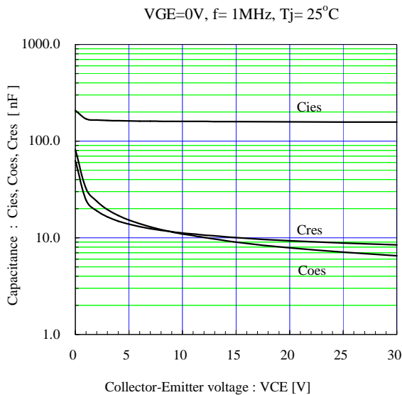
Capacitance vs. Collector-Emitter voltage (typ.)
