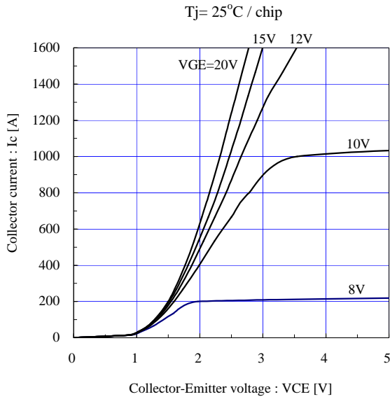
Collector current vs. Collector-Emitter voltage (typ.)
