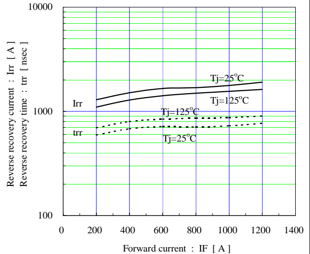
Reverse recovery characteristics (typ.) Vcc=1800V, VGE=±15V, Rg=2.4Ω
