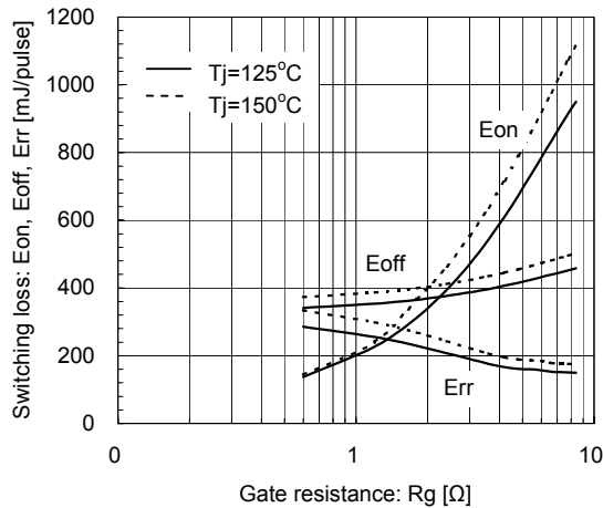
Switching loss vs. Gate resistance (typ.)(b) V_{cc}=900V, I_c=1000A, V_{ge}=\pm 15V, T_j=125^\circ C, 150^\circ C
