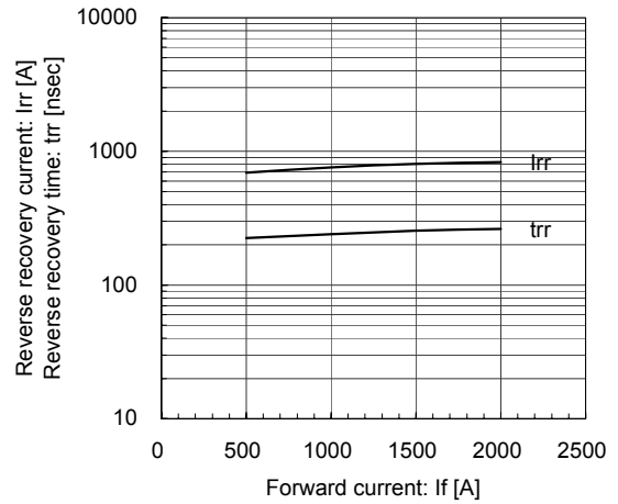
Reverse Recovery Characteristics (typ.) Vcc=900V, Vge=±15V, Rg=+1.2/-1.8Ω, Tj=25°C
