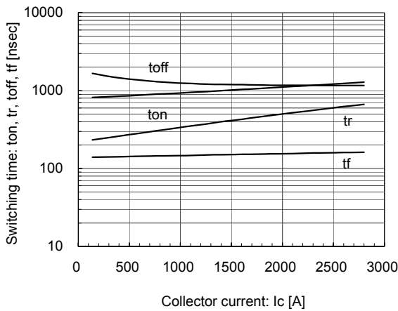
Switching time vs. Collector current (typ.) V_{cc}=600V, V_{ge}=\pm 15V, R_g=1\Omega, T_j=25^\circ C (b)
