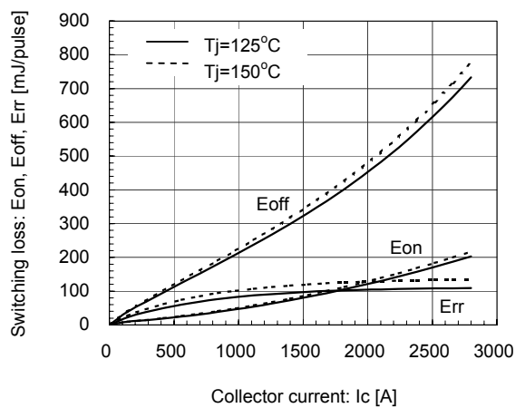
Switching loss vs. Collector current (typ.) V_{cc}=600V, V_{ge}=\pm 15V, R_g=1\Omega, T_j=125^\circ C, 150^\circ C (b)
