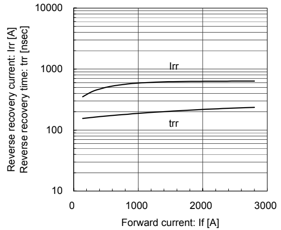
Reverse Recovery Characteristics (typ.) Vcc=600V, Vge=±15V, Rg=1Ω, Tj=25°C (b)
