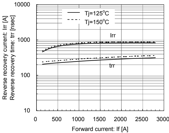
Reverse Recovery Characteristics (typ.) Vcc=600V, Vge=±15V, Rg=1Ω, Tj=125°C, 150°C (b)
