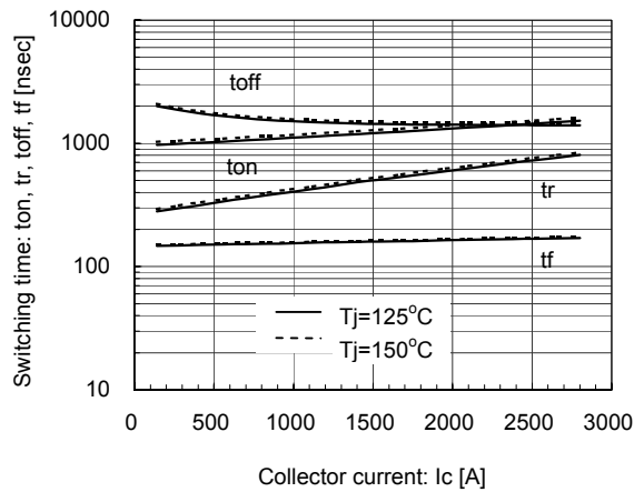
Switching time vs. Collector current (typ.) V_{cc}=600V, V_{ge}=\pm 15V, R_g=1\Omega, T_j=125^\circ C, 150^\circ C (b)
