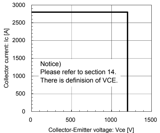
Reverse bias safe operating area (max.) +V_{ge}=15V, -V_{ge}=15V, R_g=1\Omega, T_j=150^\circ C (b)
