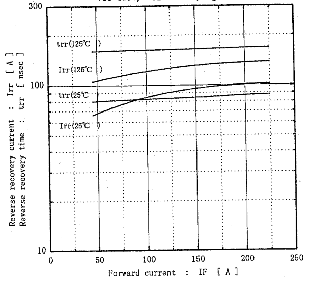
Reverse recovery characteristics (typ.) Vcc=600V, VGE=±15V, Rg=5.6Ω
