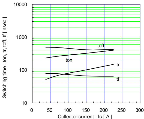
Switching time vs. Collector current (typ.) V_{cc}=600V, V_{GE}=\pm 15V, R_G=4.7\Omega, T_j=25^\circ C
