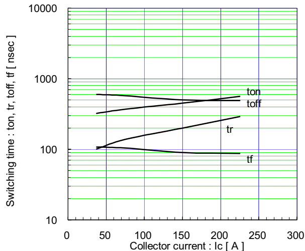
Switching time vs. Collector current (typ.) V_{cc}=600V, V_{GE}=\pm 15V, R_G=4.7\Omega, T_j=125^\circ C
