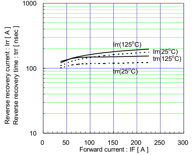
Reverse recovery characteristics (typ.) Vcc=600V, VGE=±15V, RG=4.7Ω
