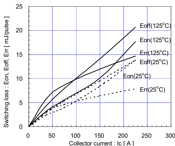
Switching loss vs. Collector current (typ.) V_{cc}=600V, V_{GE}=\pm 15V, R_G=4.7\Omega
