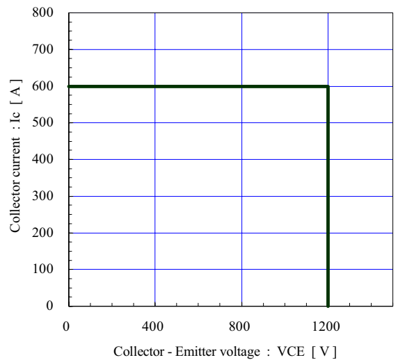
Reverse bias safe operating area +V_{GE}=15V, -V_{GE}\leq 15V, R_g\geq 1.1\Omega, T_j\leq 125^\circ C
