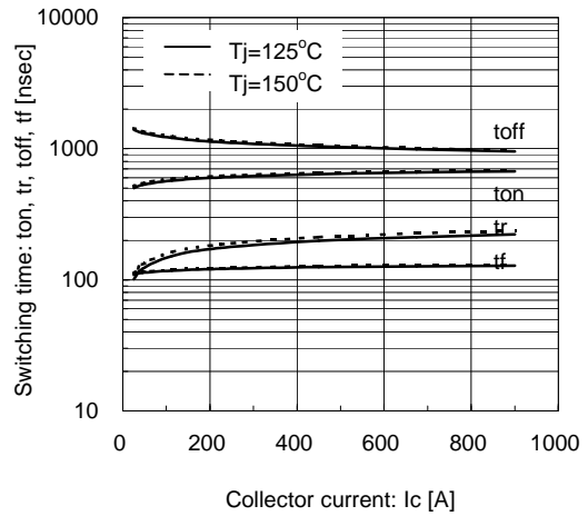
Switching time vs. Collector current (typ.) V_{cc}=600V, V_{GE}=\pm 15V, R_g=0.52\Omega, T_j=125^\circ C, 150^\circ C
