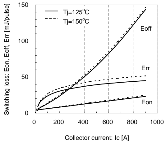
Switching loss vs. Collector current (typ.) V_{cc}=600, V_{GE}=\pm 15V, R_g=0.52\Omega, T_j=125^\circ C, 150^\circ C
