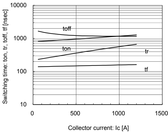
Switching time vs. Collector current (typ.) V_{cc}=600V, V_{ge}=\pm 15V, R_g=2.4\Omega, T_j=25^\circ C
