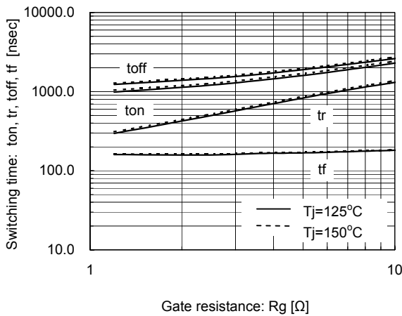
Switching time vs. Gate resistance (typ.) V_{cc}=600V, I_c=600A, V_{ge}=\pm 15V, T_j=125^\circ C, 150^\circ C
