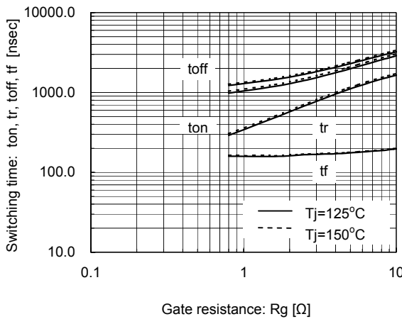
Switching time vs. Gate resistance (typ.) V_{cc}=600V, I_c=900A, V_{ge}=\pm 15V, T_j=125^\circ C, 150^\circ C
