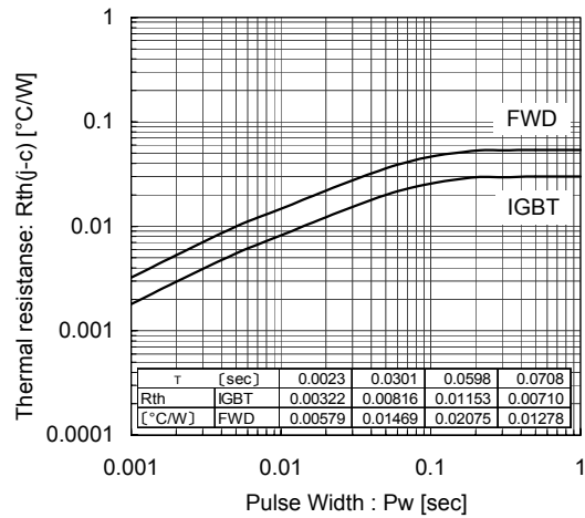
Transient Thermal Resistance (max.)(a)
