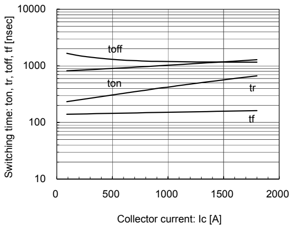
Switching time vs. Collector current (typ.) V_{cc}=600V, V_{ge}=\pm 15V, R_g=1.6\Omega, T_j=25^\circ C
