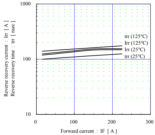
Reverse recovery characteristics (typ.) Vcc=600V, VGE=±15V, Rg=4.7Ω
