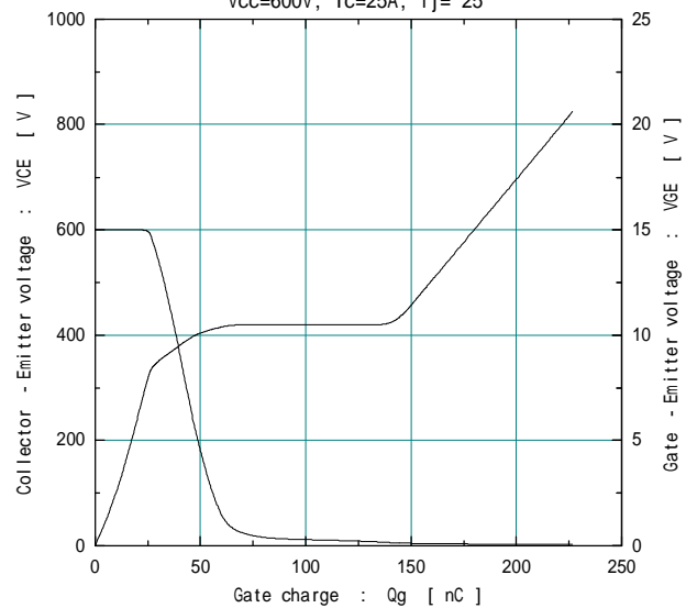
Dynamic Gate charge (typ.) Vcc=600V, Ic=25A, Tj= 25
