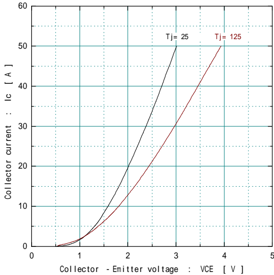
Collector current vs. Collector-Emittor voltage VGE=15V (typ.)
