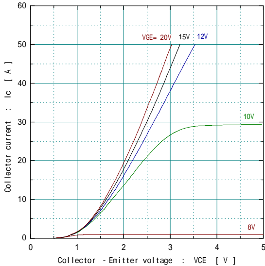
Collector current vs. Collector-Emittor voltage Tj= 25 (typ.)
