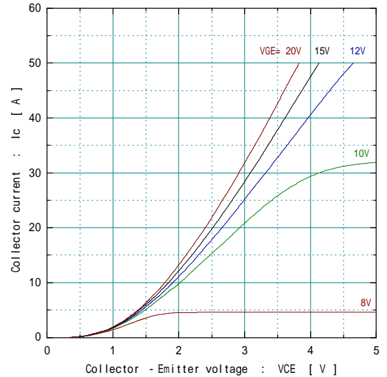
Collector current vs. Collector-Emittor voltage Tj= 125 (typ.)
