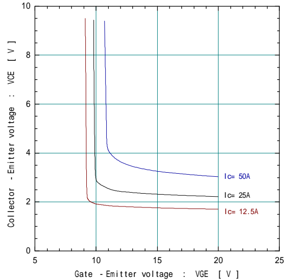
Collector-Emittor voltage vs. Gate-Emittor voltage Tj= 25 (typ.)
