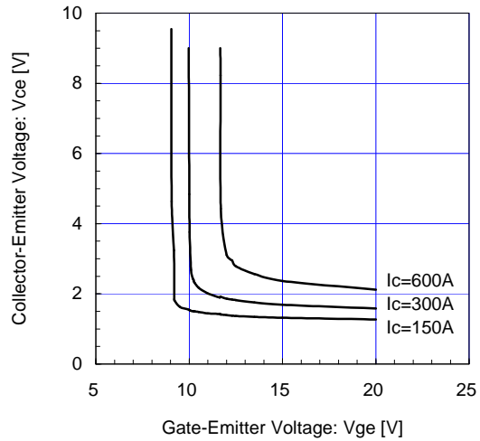
Collector-Emittter voltage vs. Gate-Emittter voltage (typ.) T j = 25°C / chip
