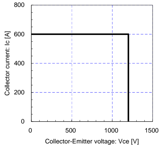
Reverse bias safe operating area (max.) +V_{ge}=15V, -V_{ge}\le 15V, R_g\ge 0.93\Omega, T_j=150^\circ C
