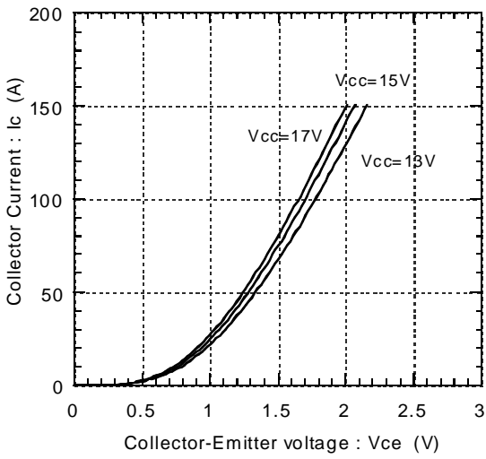
Collector current vs. Collector-Emittter voltage T j =125°C(Chip)
