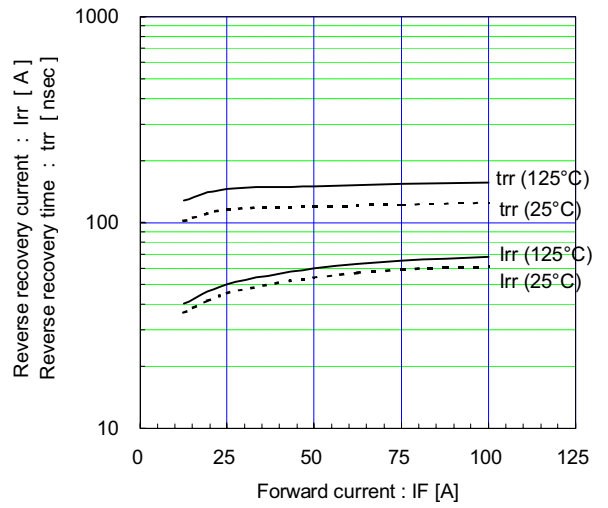
[ Inverter ] Reverse recovery characteristics (typ.) Vcc=600V, VGE=±15V, Rg=9.1Ω
