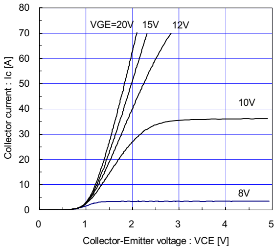
[ Brake ] Collector current vs. Collector-Emittor voltage (typ.) T_j = 25^\circ\text{C} / chip
