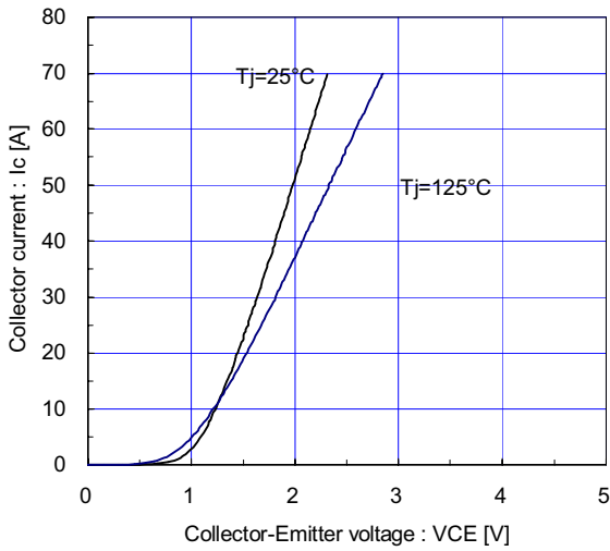
[ Brake ] Collector current vs. Collector-Emittor voltage (typ.) V_{GE} = 15\text{V} / chip
