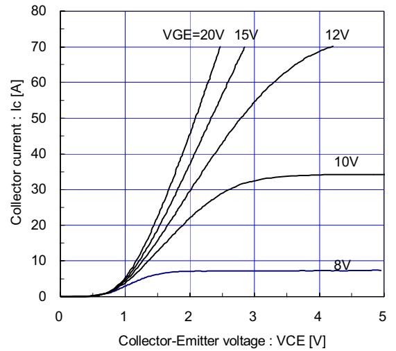
[ Brake ] Collector current vs. Collector-Emittor voltage (typ.) T_j = 125^\circ\text{C} / chip
