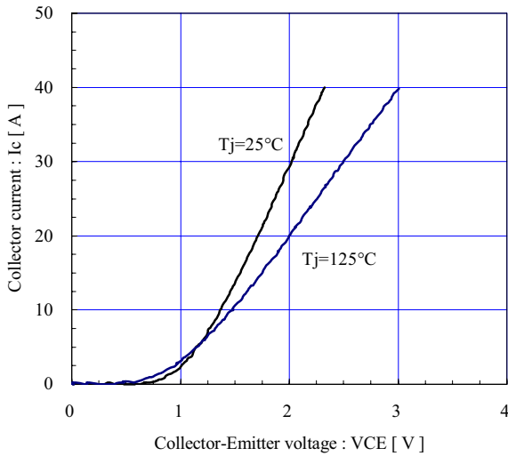
[ Brake ] Collector current vs. Collector-Emitter voltage (typ.) V_{GE} = 15\text{V} / chip
