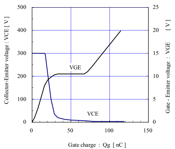
[ Inverter ] Dynamic Gate charge (typ.) V_{CC} = 300\text{V}, I_c = 30\text{A}, T_j = 25^\circ\text{C}
