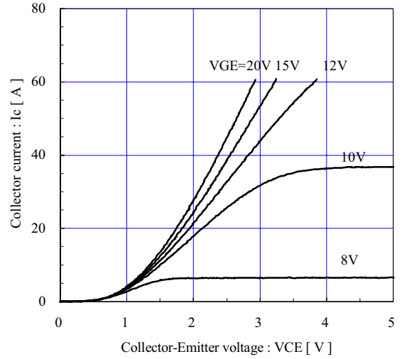
[ Inverter ] Collector current vs. Collector-Emittor voltage (typ.) T_j = 125^\circ\text{C} / \text{chip}
