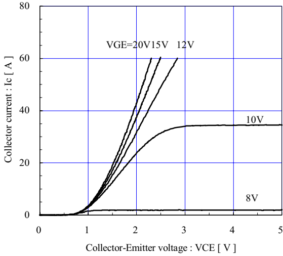
[ Inverter ] Collector current vs. Collector-Emittor voltage (typ.) T_j = 25^\circ\text{C} / \text{chip}
