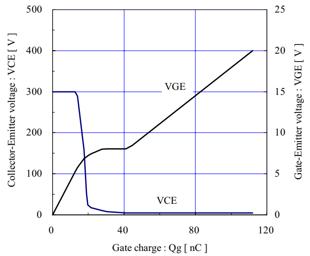
[ Brake ] Dynamic Gate charge (typ.) V_{CC} = 300\text{V} , I_C = 20\text{A} , T_j = 25^\circ\text{C}
