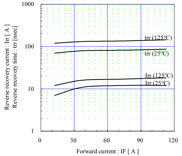
[ Inverter ] Reverse recovery characteristics (typ.) Vcc=300V, VGE=±15V, Rg=47Ω
