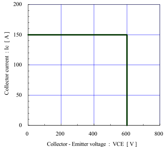
[ Inverter ] Reverse bias safe operating area (max.) +V_{GE}=15V, -V_{GE} \le 15V, R_g \ge 47\Omega, T_j \le 125^\circ C
