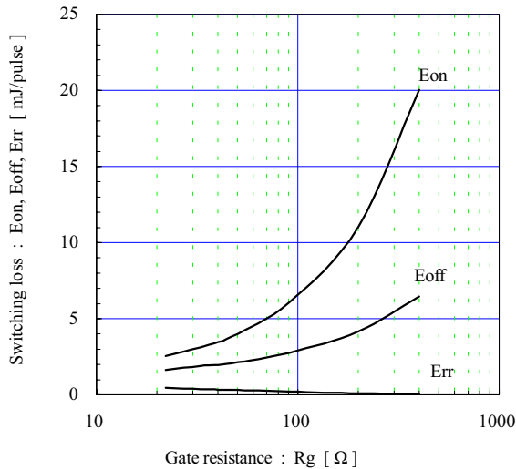
[ Inverter ] Switching loss vs. Gate resistance (typ.) V_{cc}=300V, I_c=75A, V_{GE}=\pm 15V, T_j=125^\circ C
