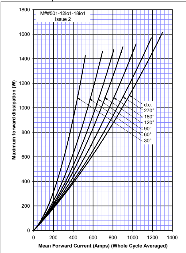
Figure 6 – On-state current vs. Power dissipation – Square wave
